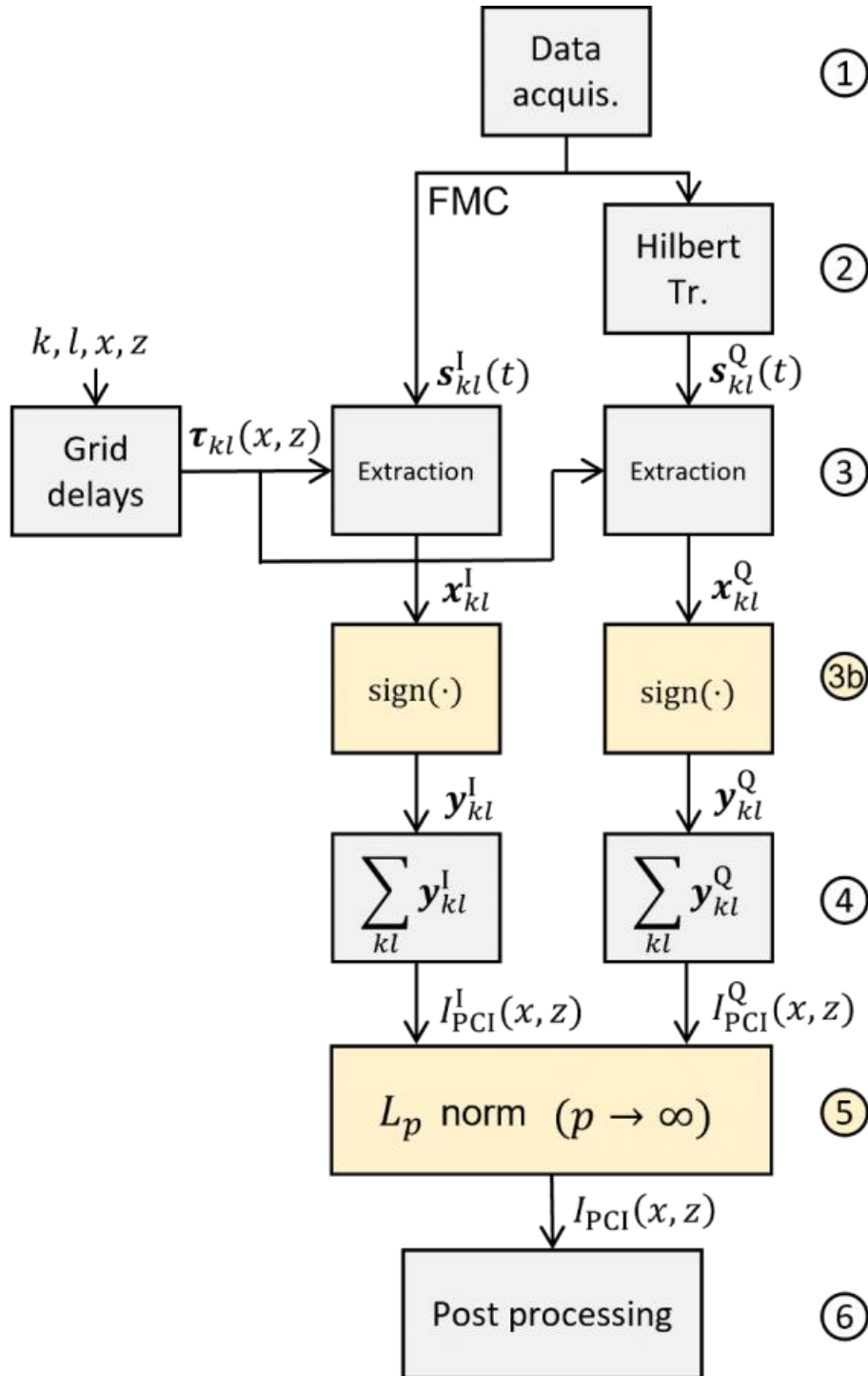
Figure 4. Principle of the PCI algorithm.
